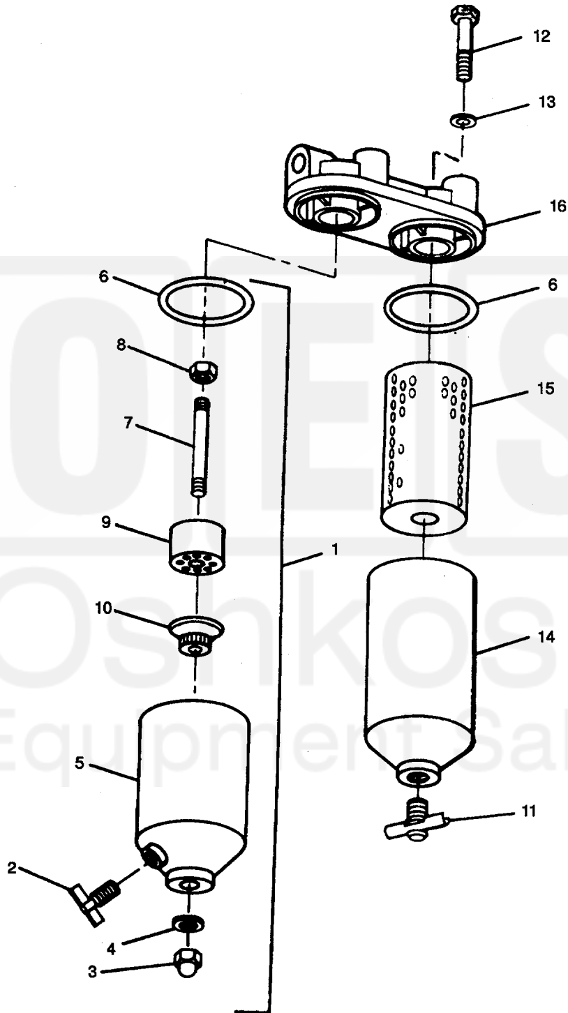
Figure 71. Filter, Fluid.
