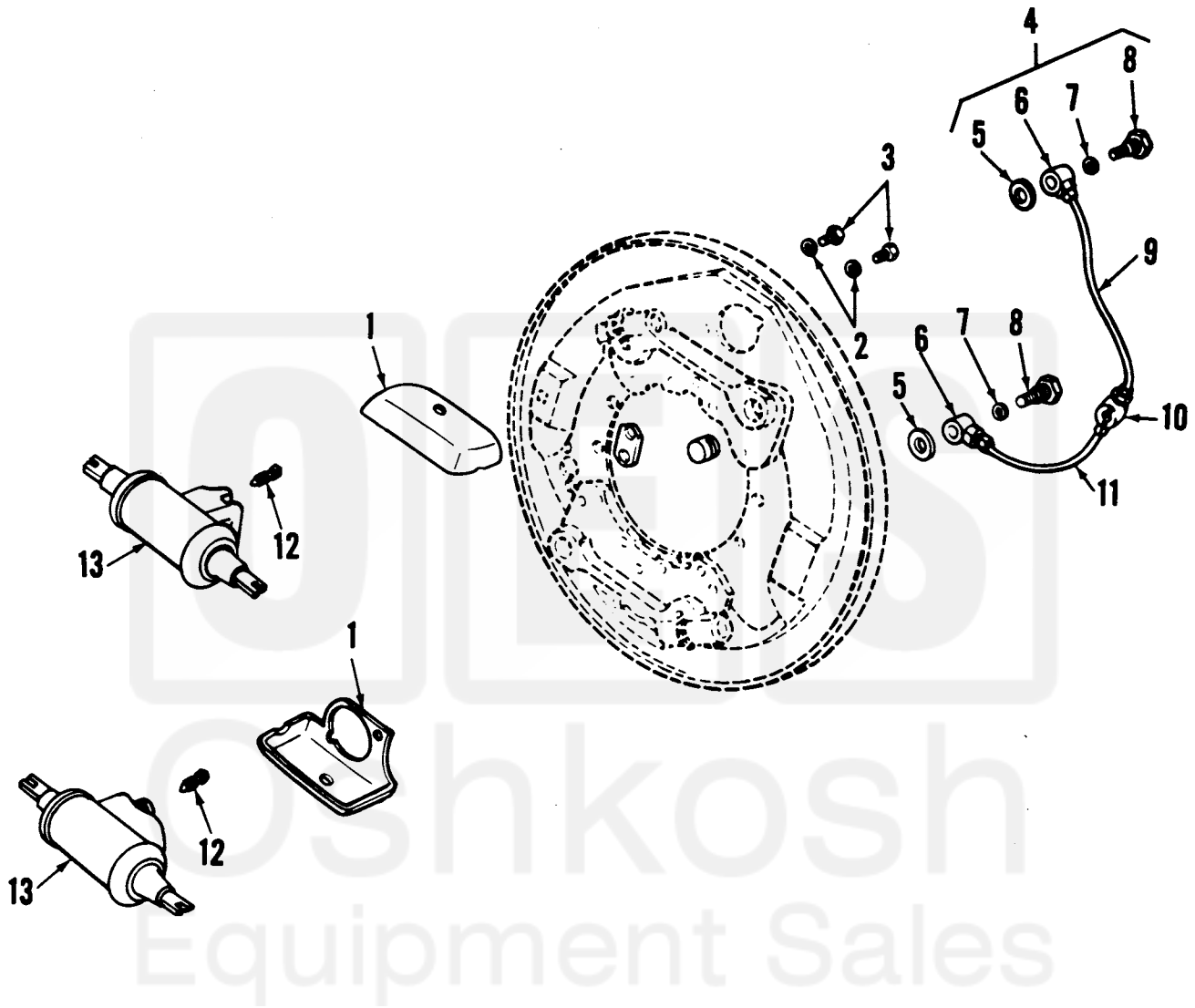
Figure 15. Wheel Cylinder and Hydraulic Tubes.
