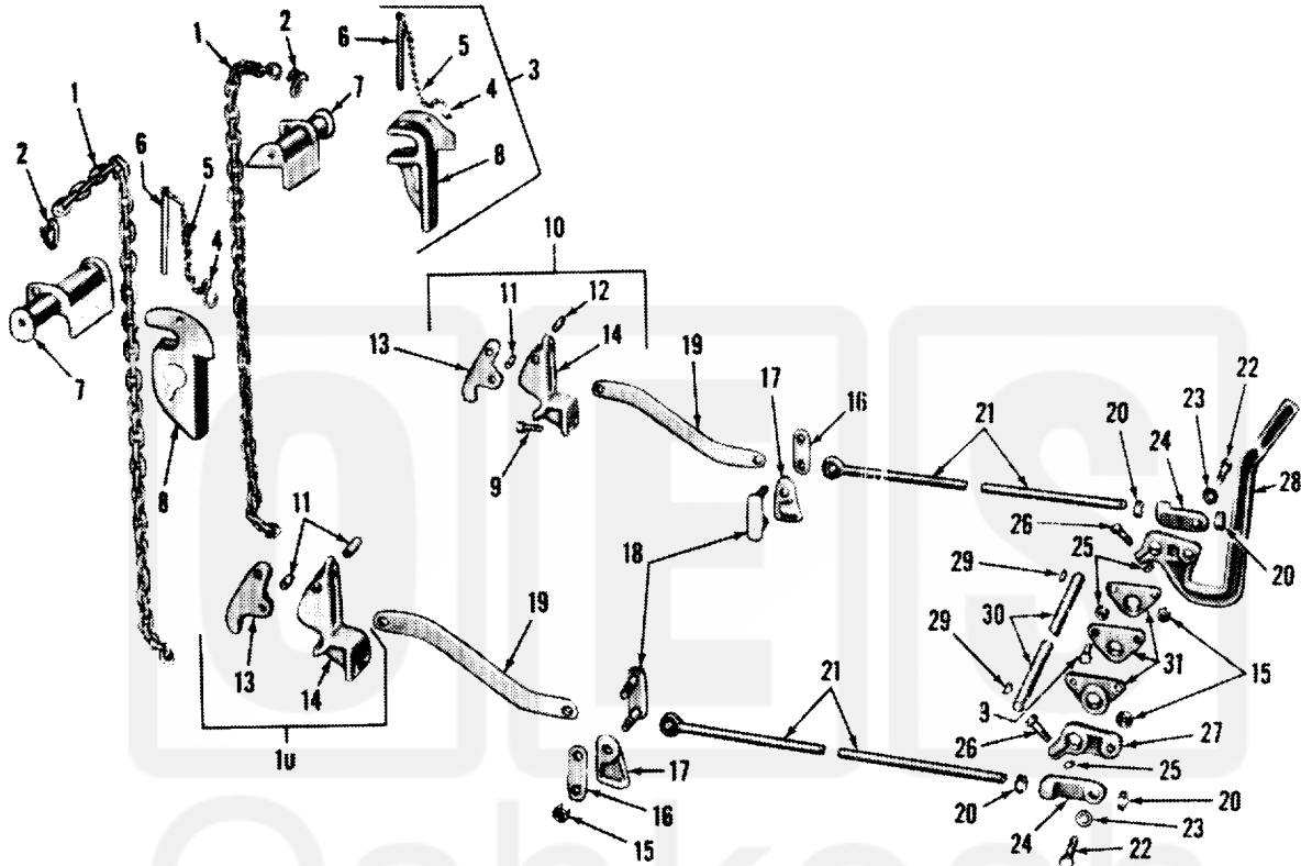
Figure 148. Dump body end gate linkage.
