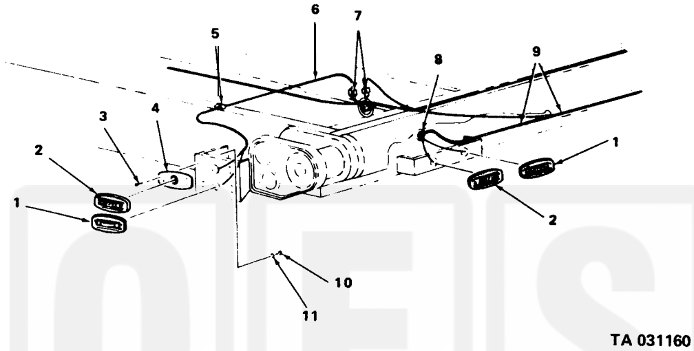
Figure 91. Rear wiring harness (M756A2).
