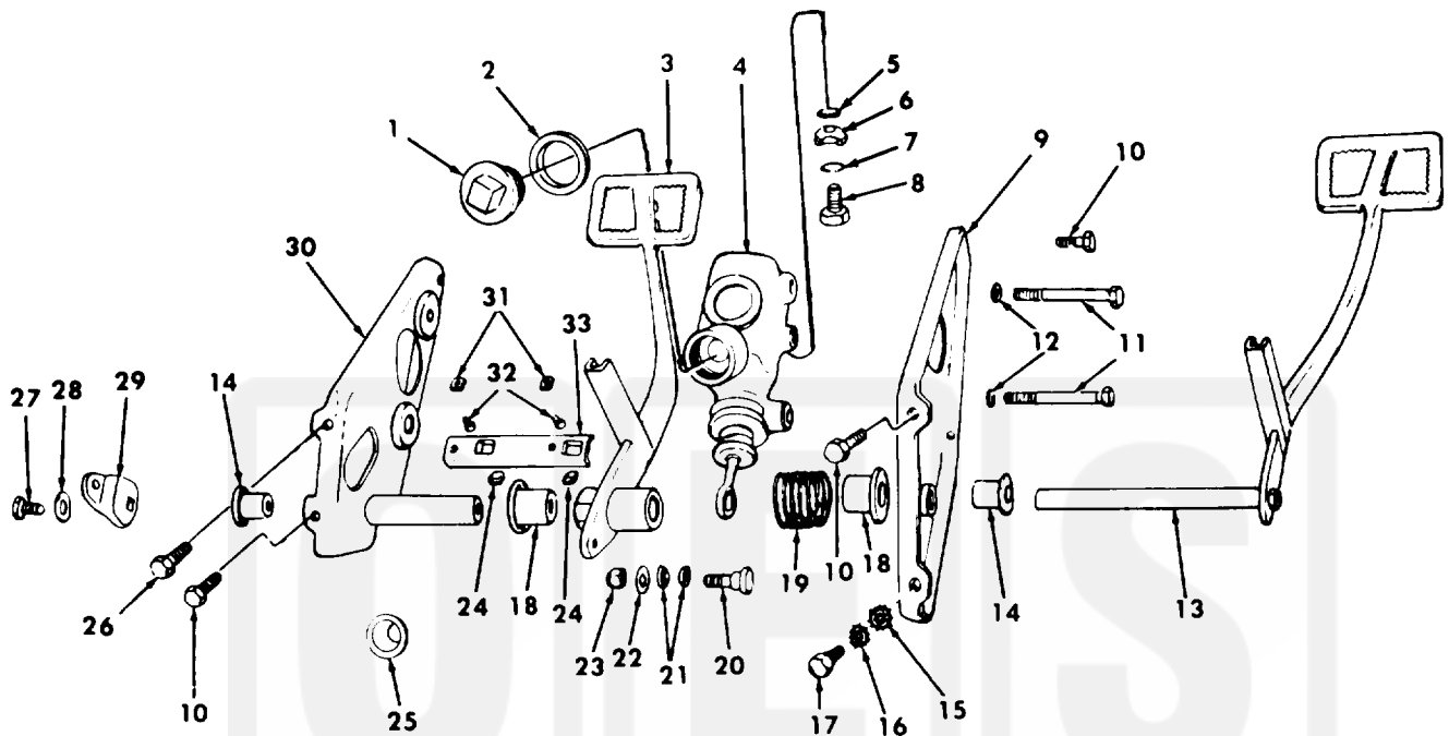
Figure 84. Master Cylinder, Brake Pedal Assembly, and Related Parts. (M151, M151A1, M151A1C, and M718 only).
