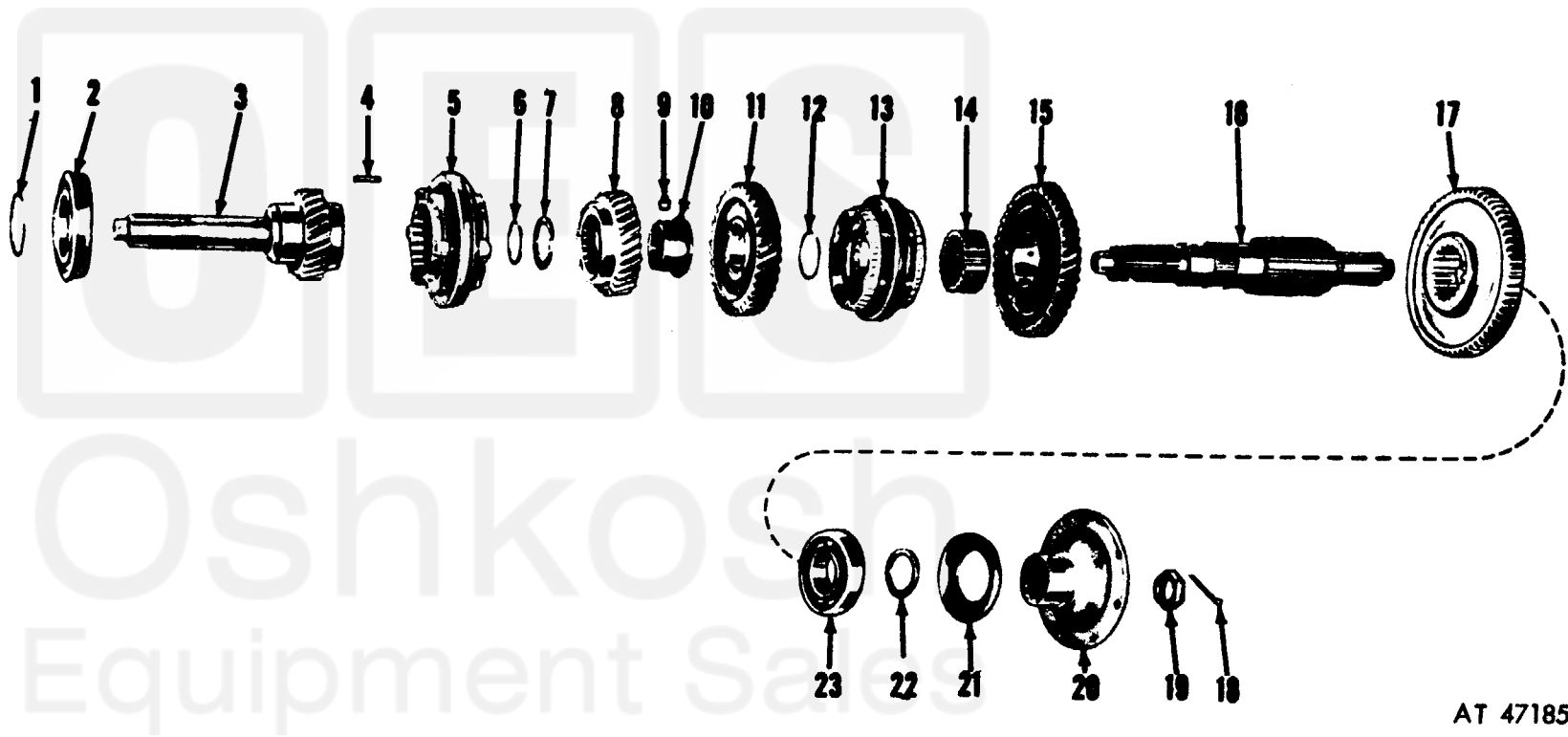
Figure 45. Transmission input shaft and main shaft with gears.
