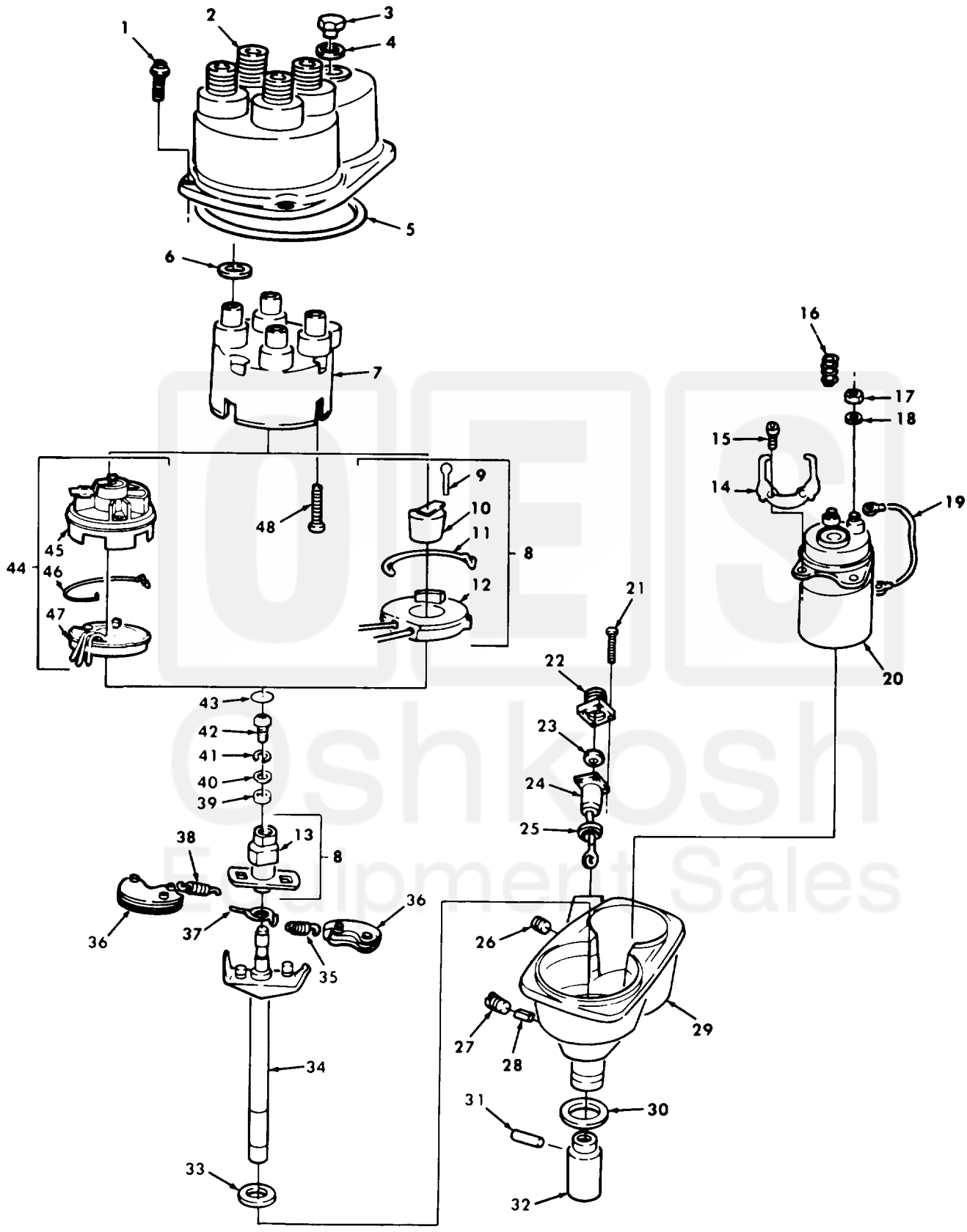
Figure 45. Distributor Assembly.
