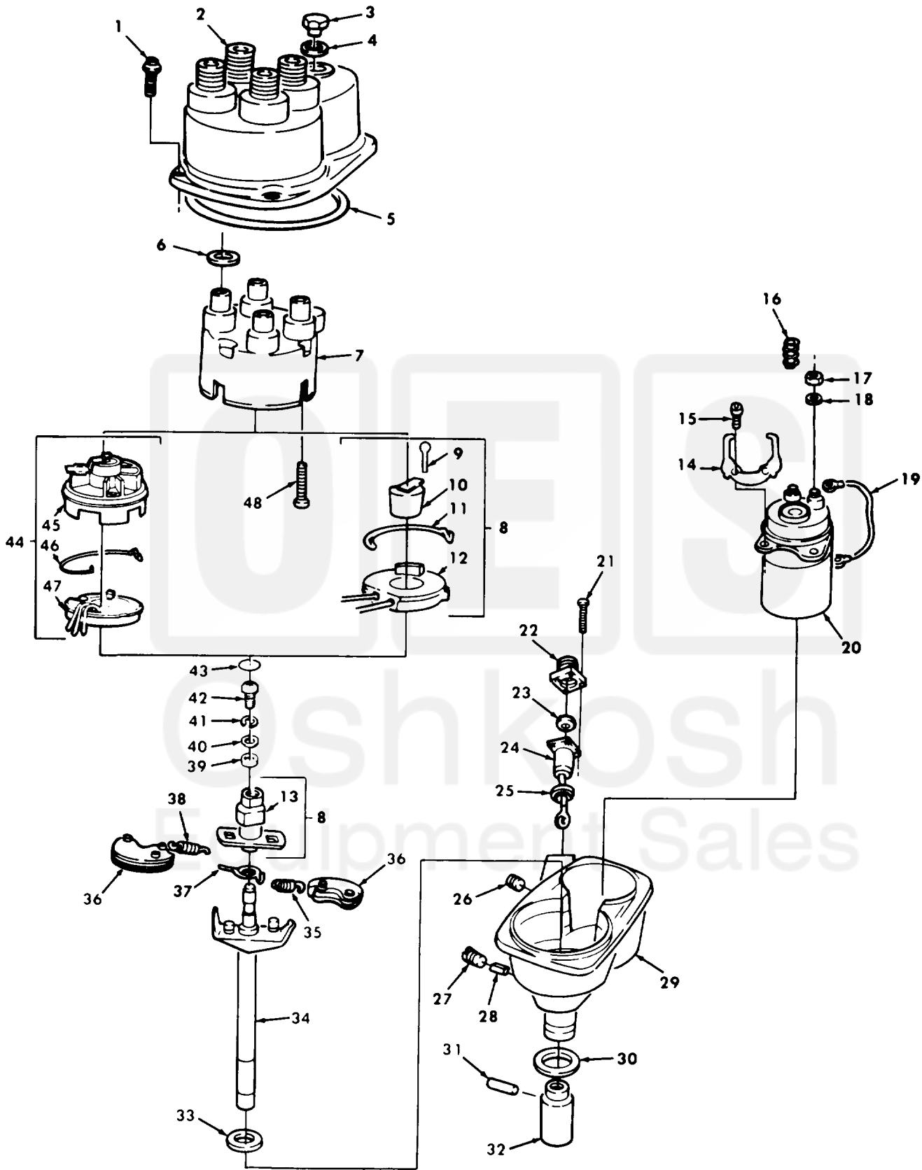
Figure 45. Distributor Assemble.
