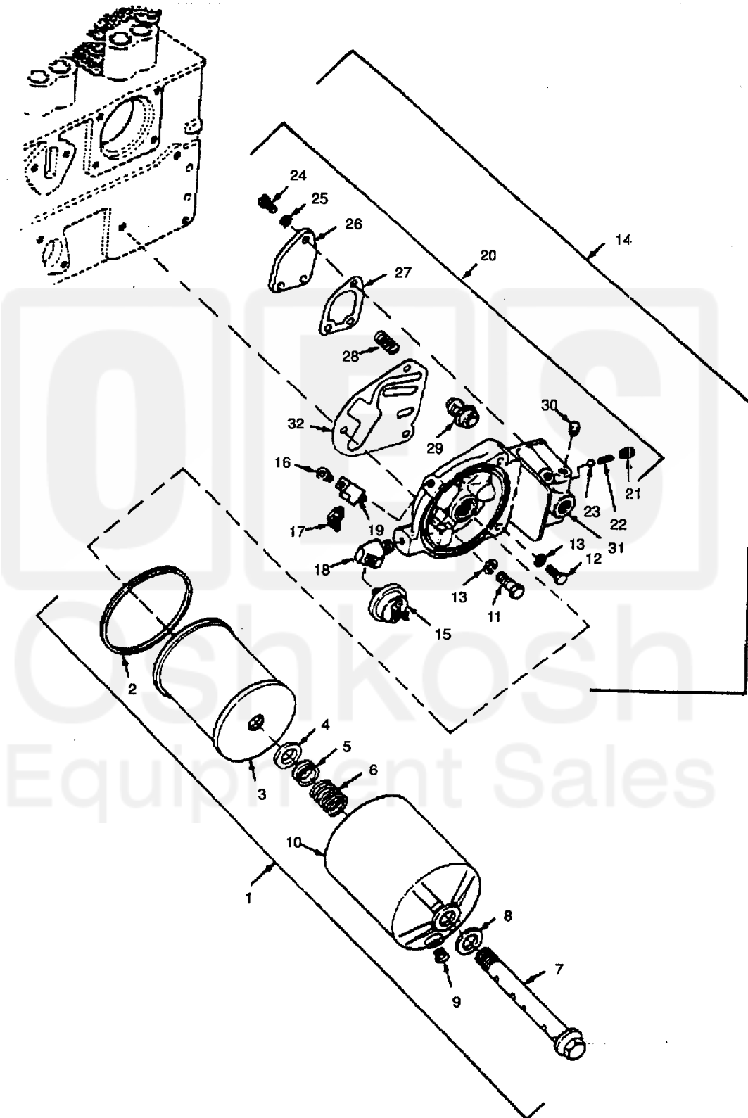
Figure 47. Oil Filter Assembly - Exploded View
