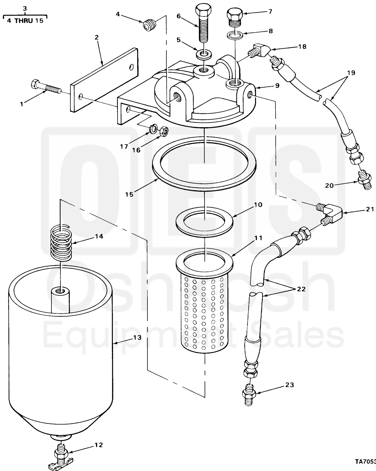
FIGURE 36. FUEL FILTER.
