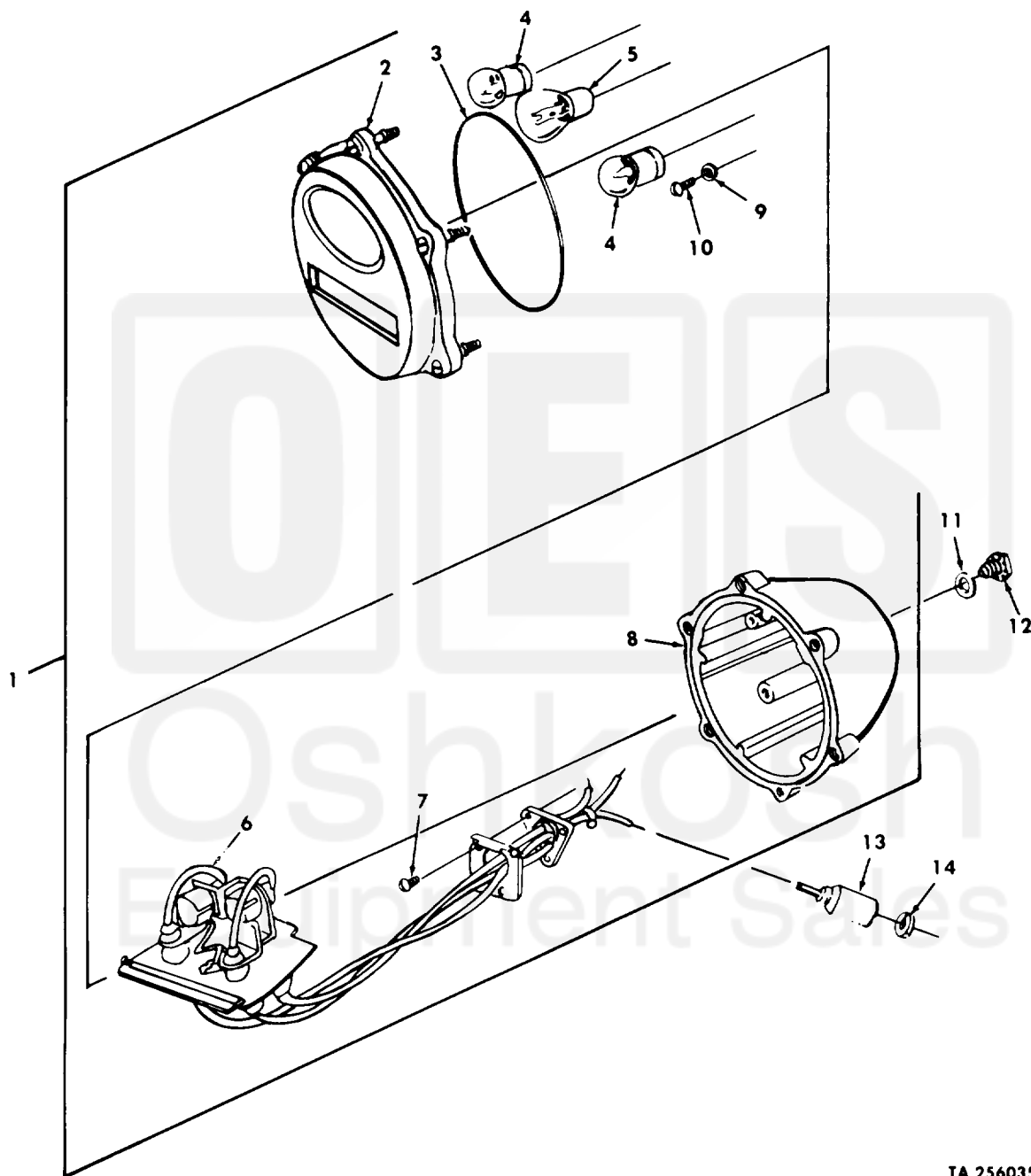
Figure 56. Taillight Assembly.
