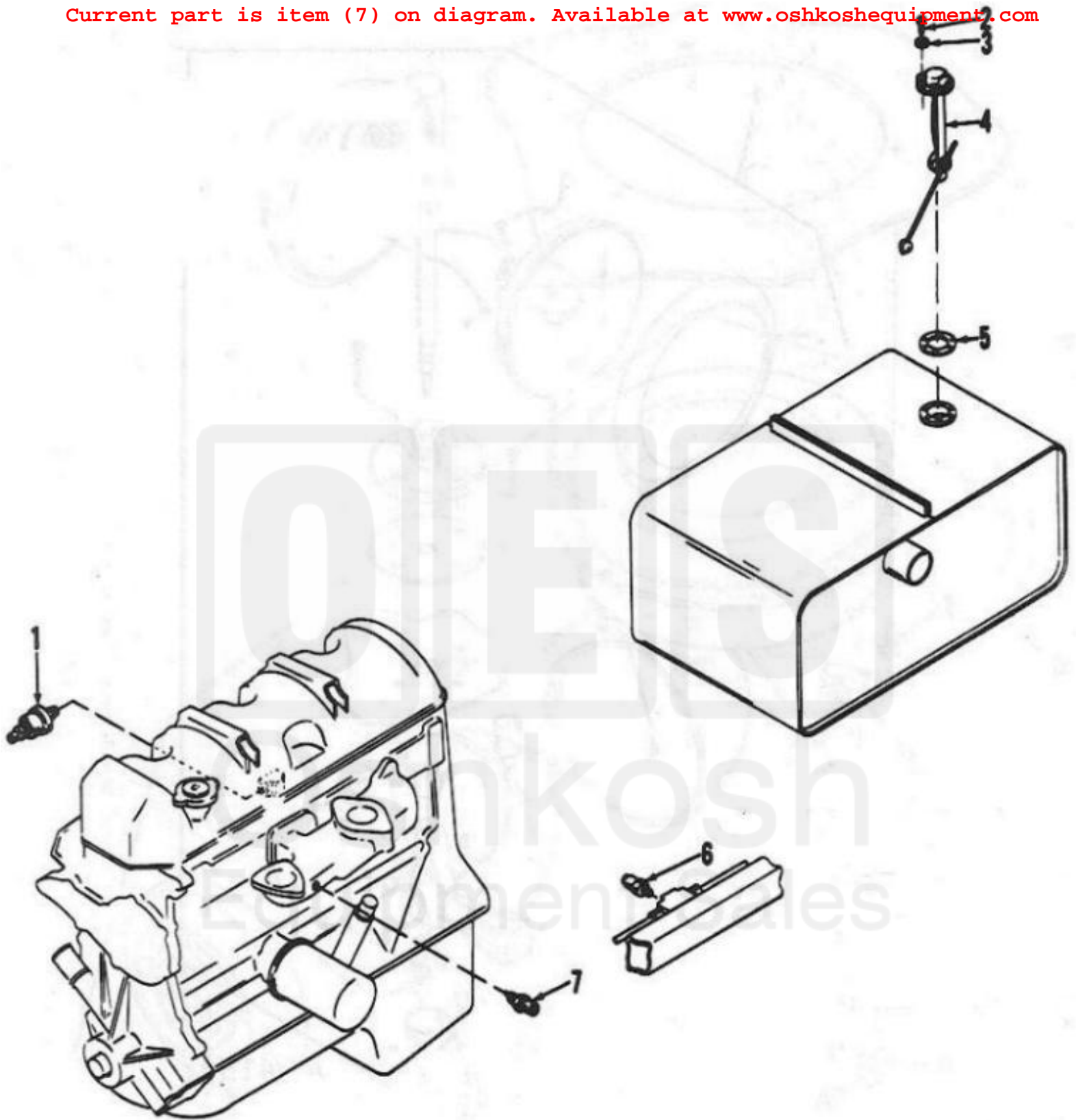
Figure 53: Sending Units
