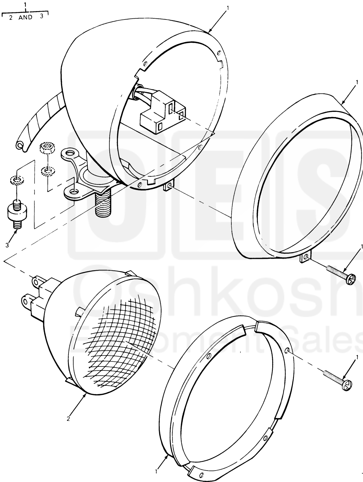
FIGURE 85. HEADLIGHT ASSEMBLY.
