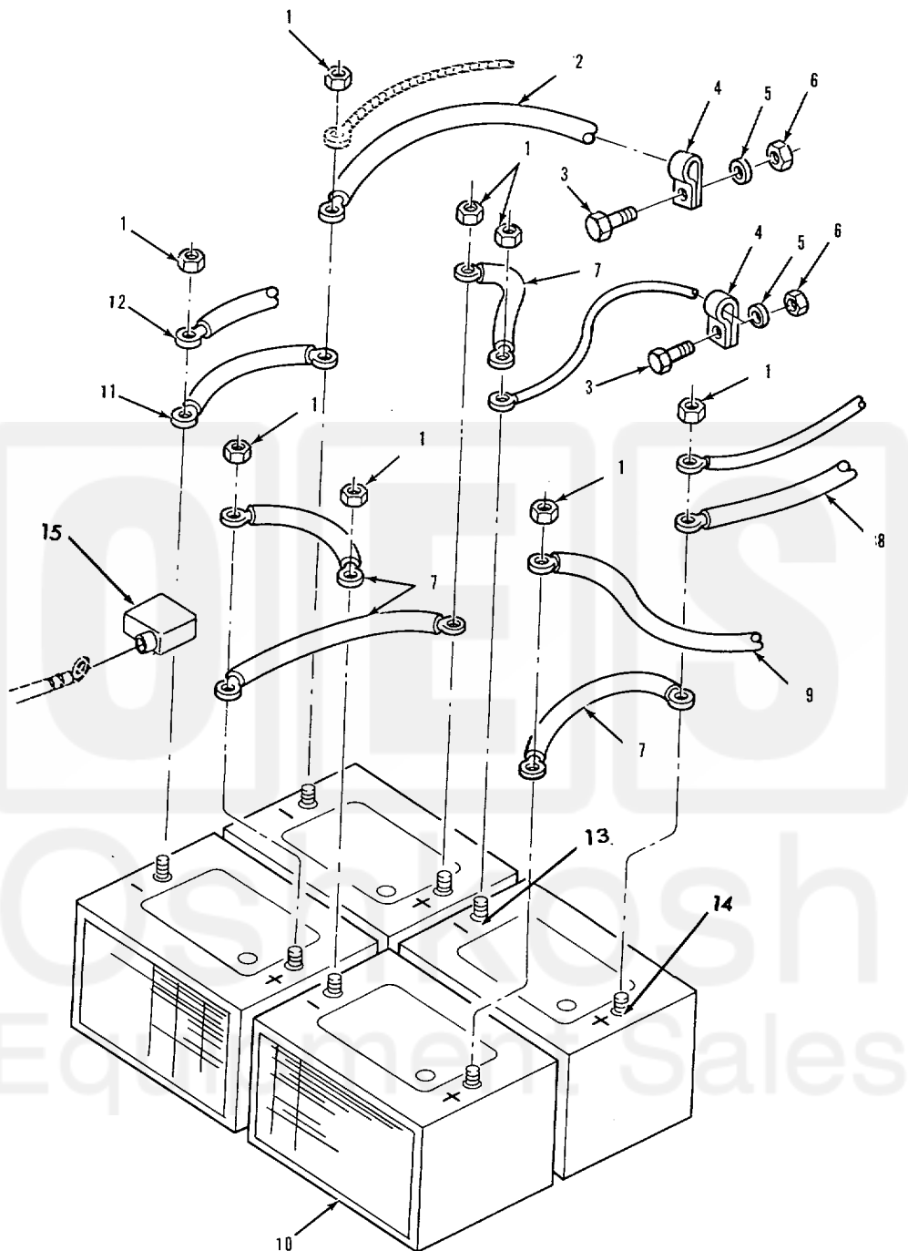
FIGURE 48. BATTERY AND RELATED PARTS.
