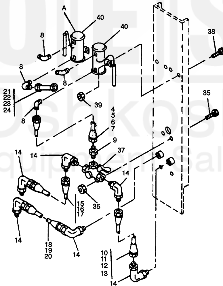
Figure 72. Center Support and Related parts (Sheet 2 of 2)
