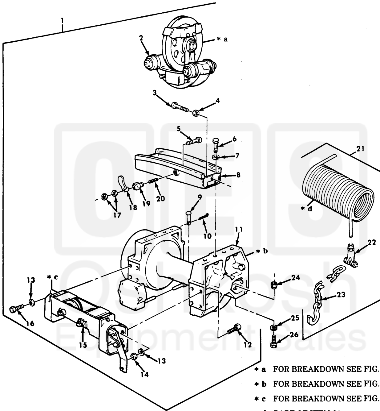
Figure 413. Wrecker Rear Winch Assembly Complete and Wire Rope Assembly.
