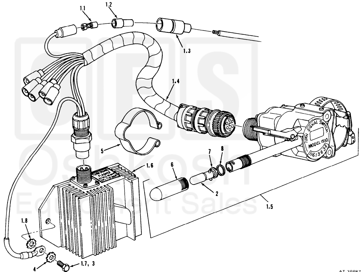
Figure 6-11. Directional control and flasher.
