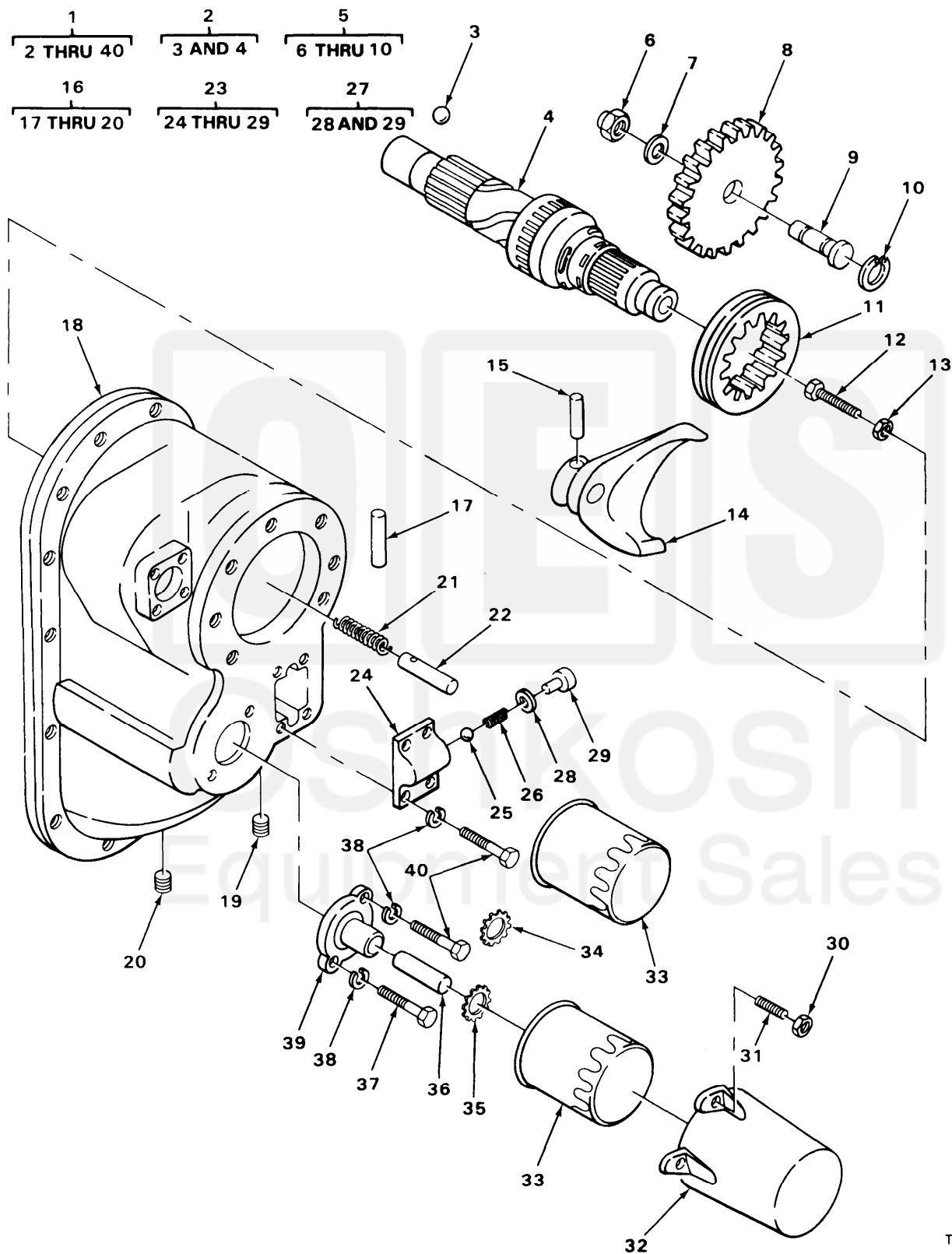
FIGURE 99 REAR COVER INPUT SHAFT AND SHIFT ASSEMBLY (MODEL M915).
