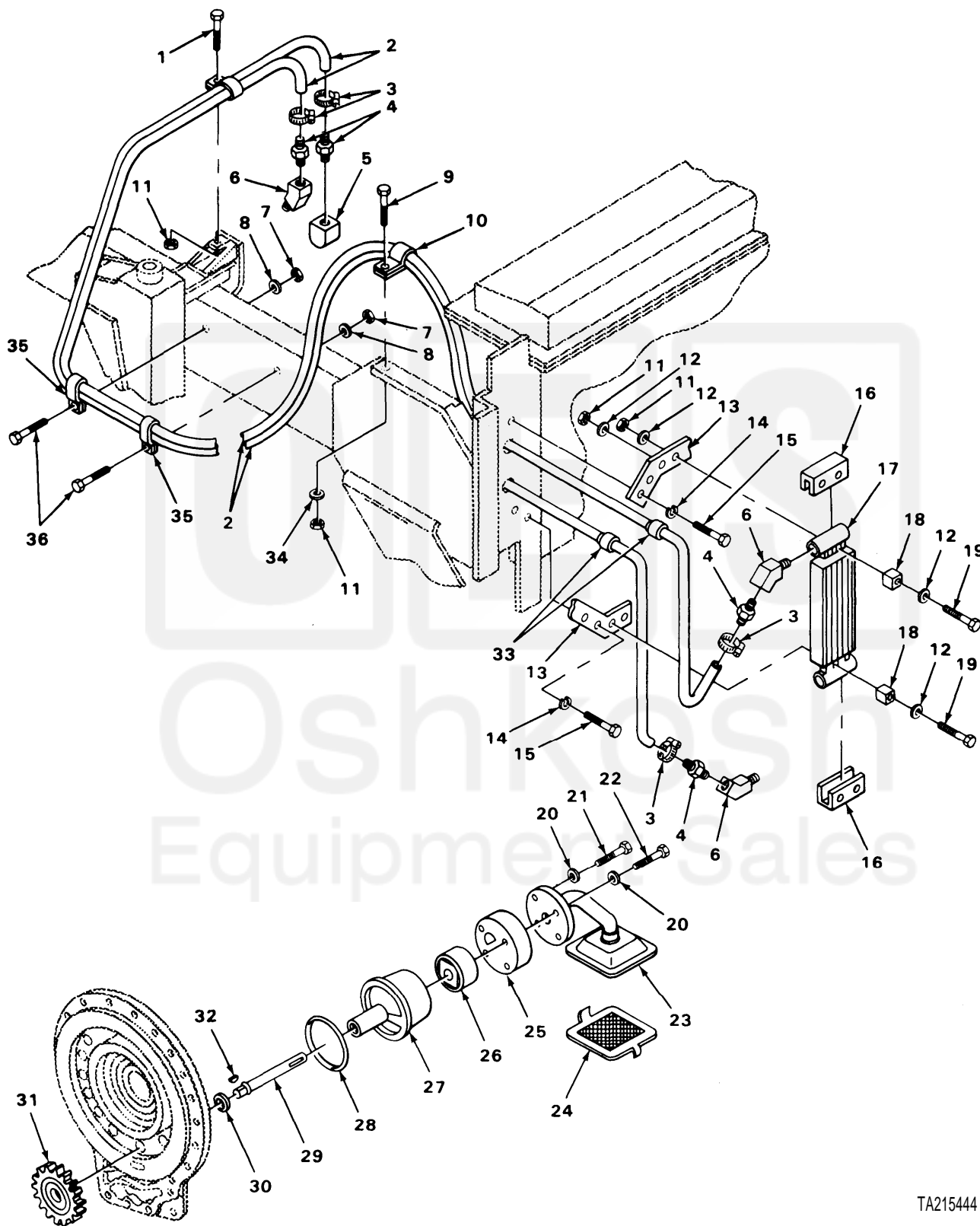
FIGURE 76. TRANSMISSION OIL PUMP COOLER AND LINES.
