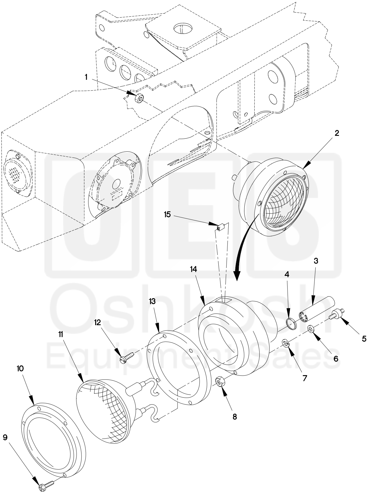
FIGURE 61. HEADLAMP ASSEMBLY
