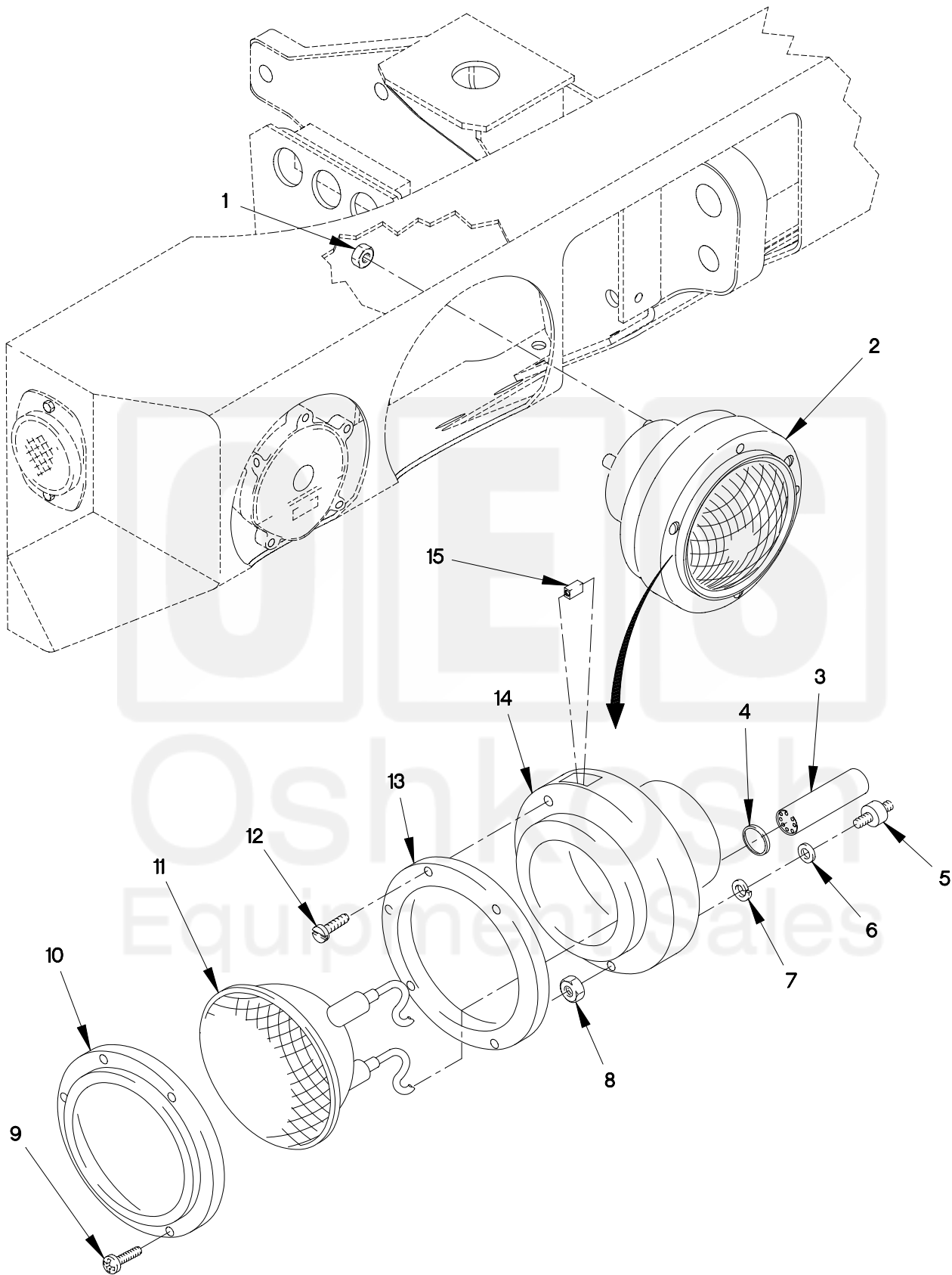
FIGURE 66. HEADLAMP ASSEMBLY
