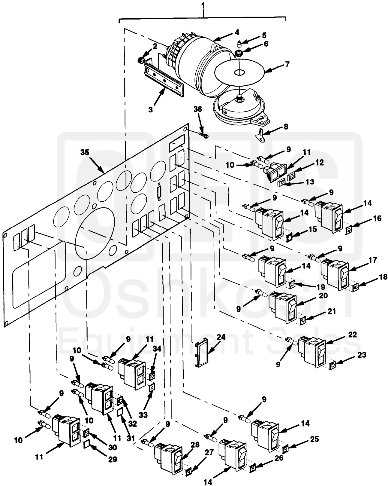
Figure 58. instrument Panel (Sheet 1 of 3)
