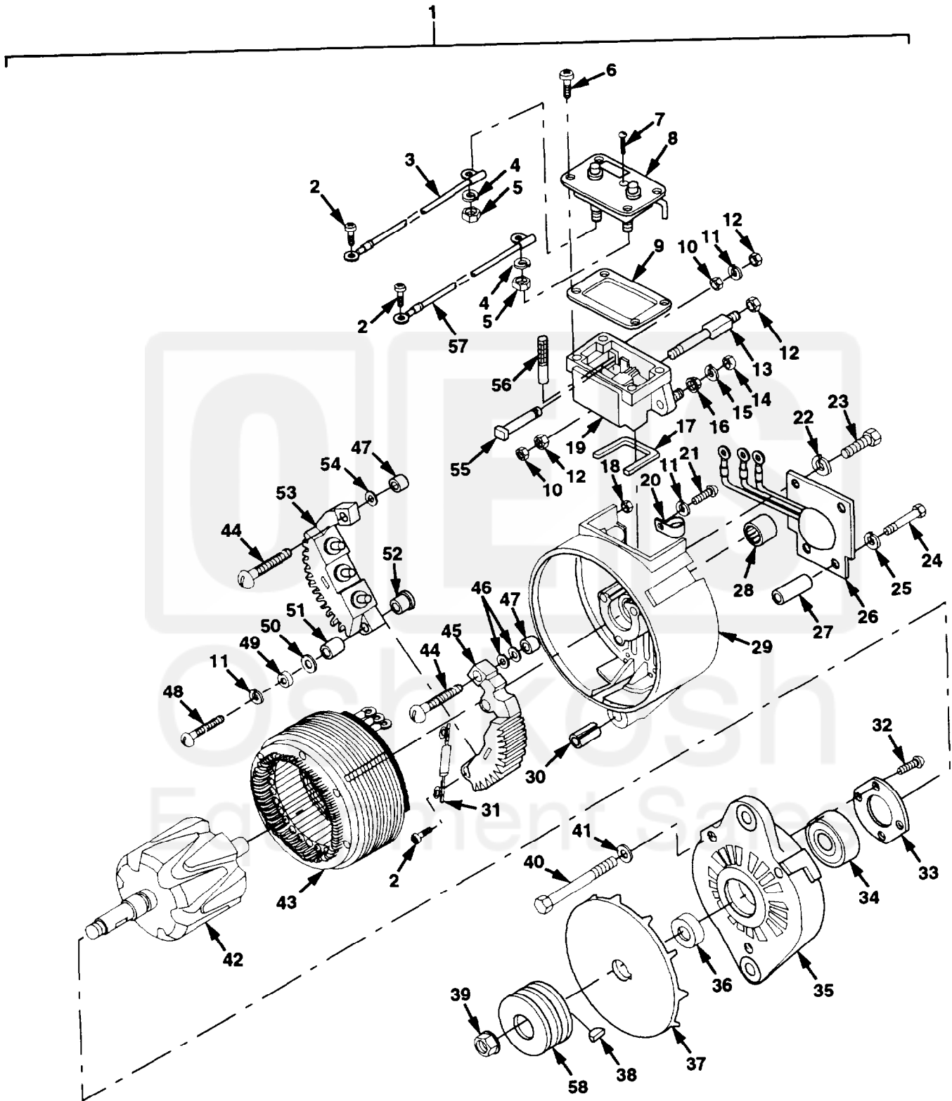
Figure 54. 24V Alternator Assembly
