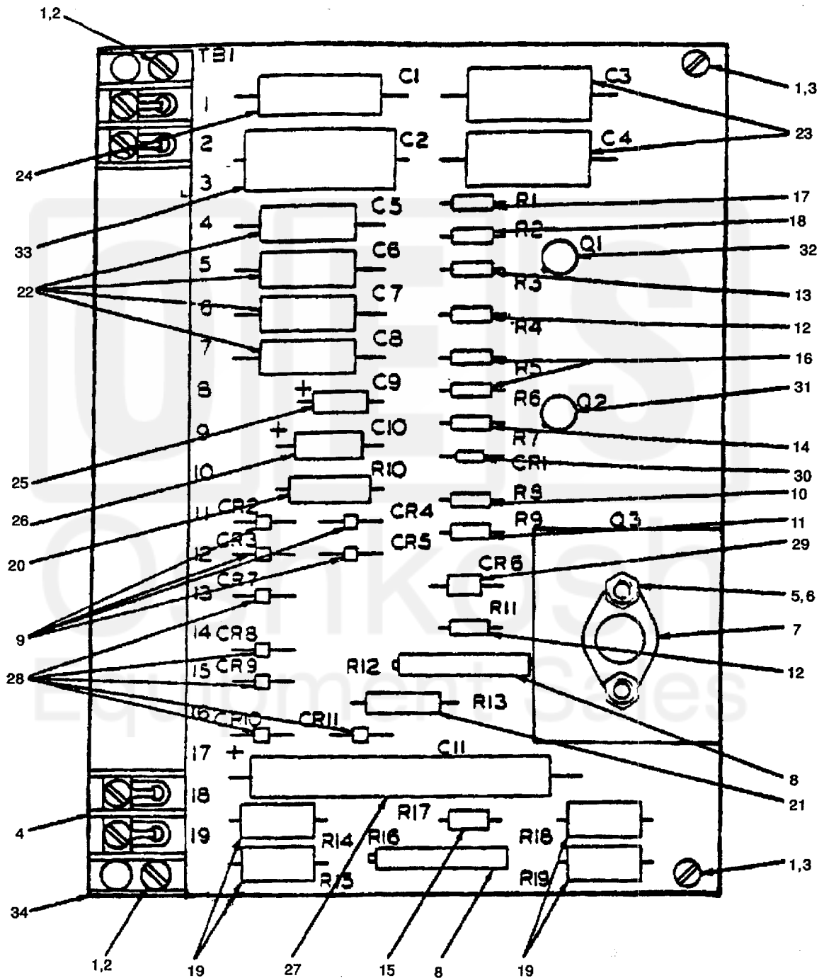
Figure 9. Voltage Regulator
