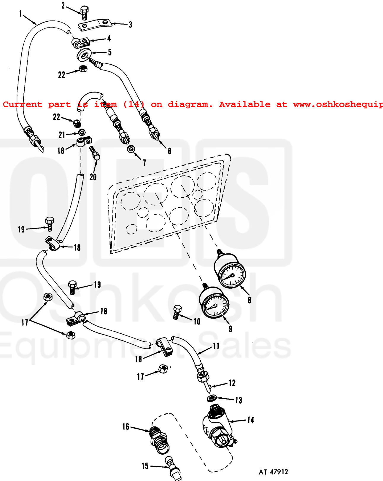
Figure 207. Speedometer and tachometer shafts and related parts.
