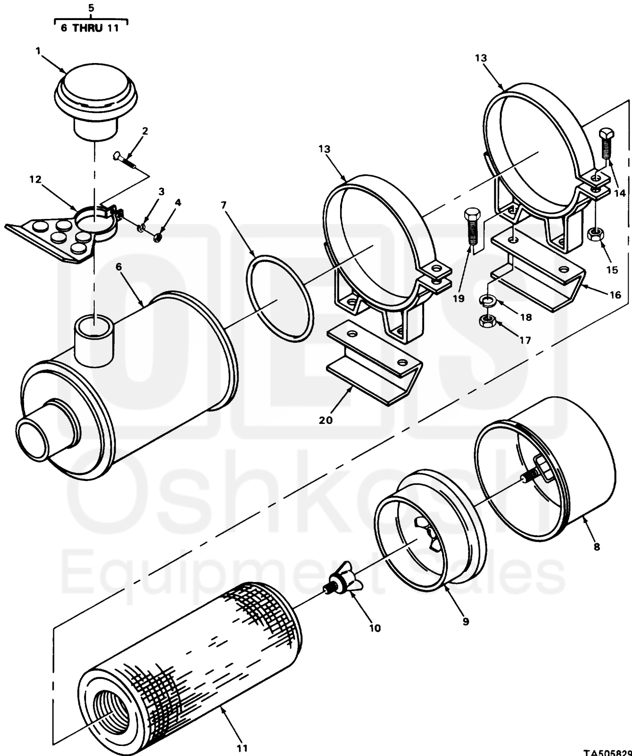
FIGURE 9. AIR CLEANER.
