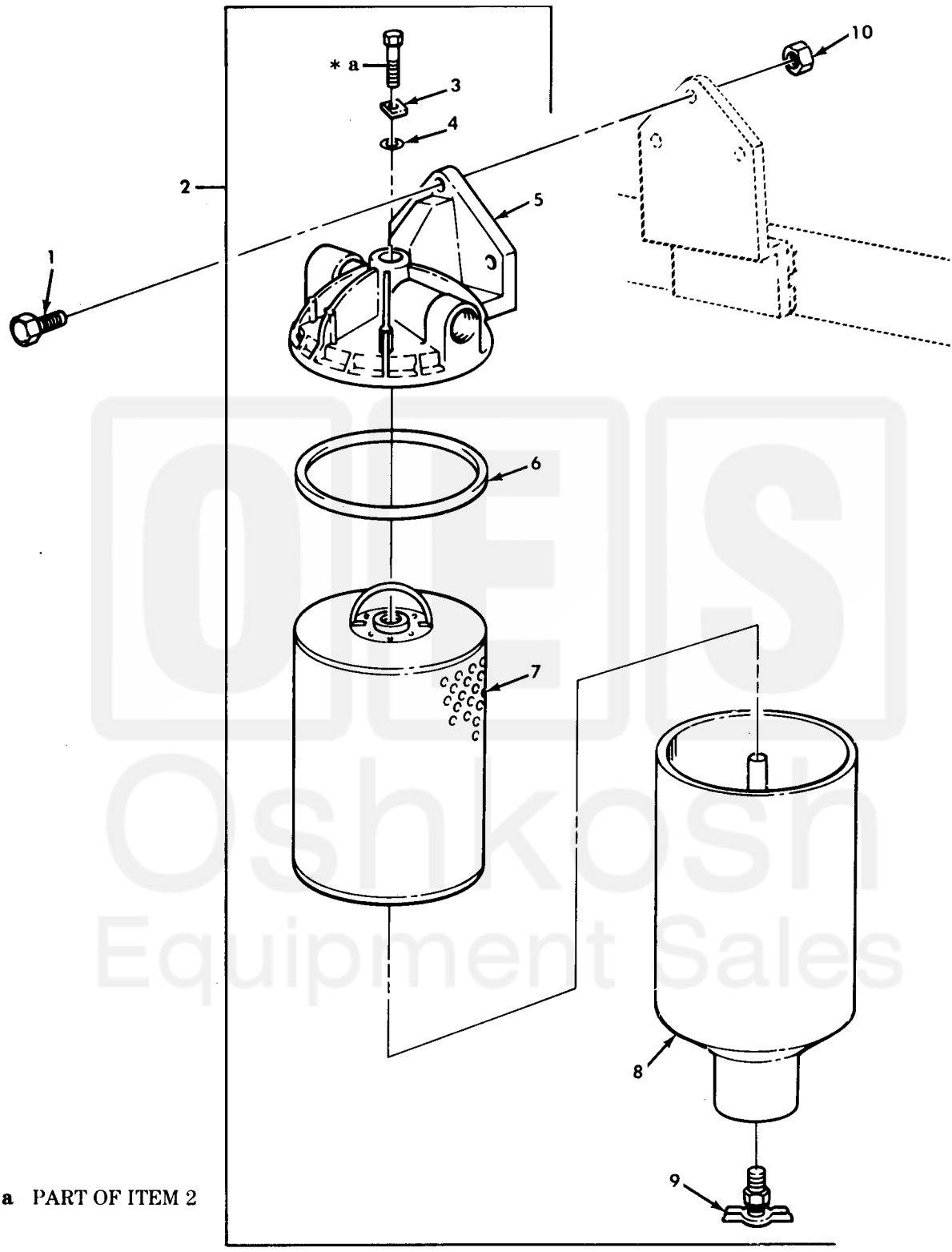
Figure 59. Fuel Filter, Water Separator, and Mounting Hardware.
