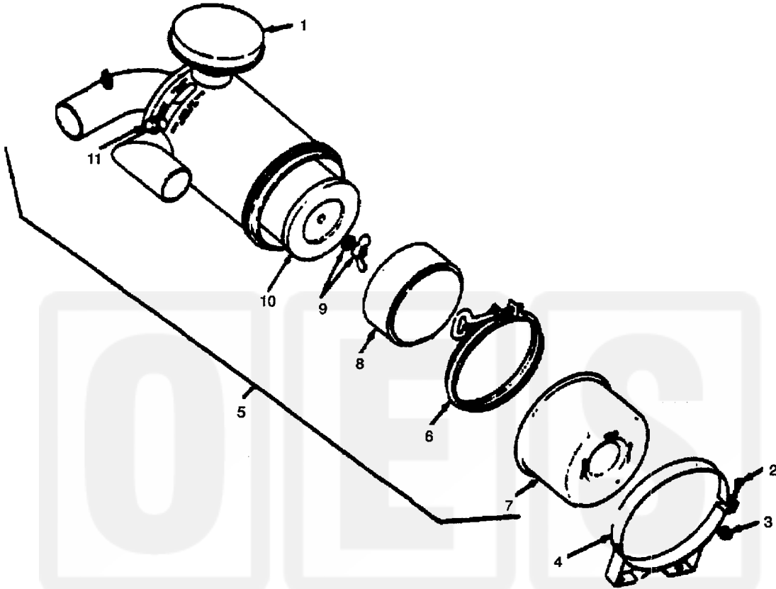
Figure 22. Air Cleaner - Exploded View
