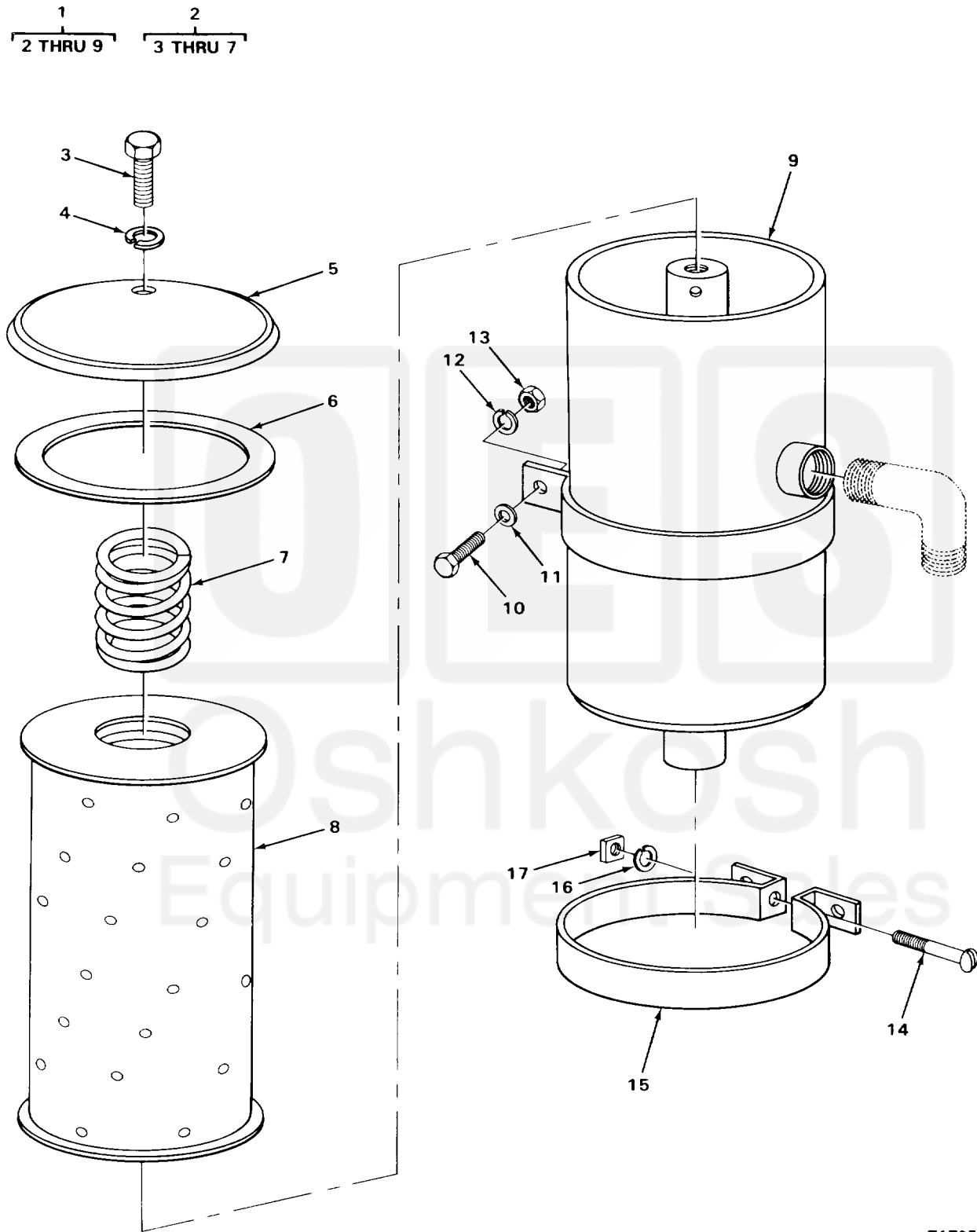
FIGURE 89. TRANSMISSION OIL FILTER
