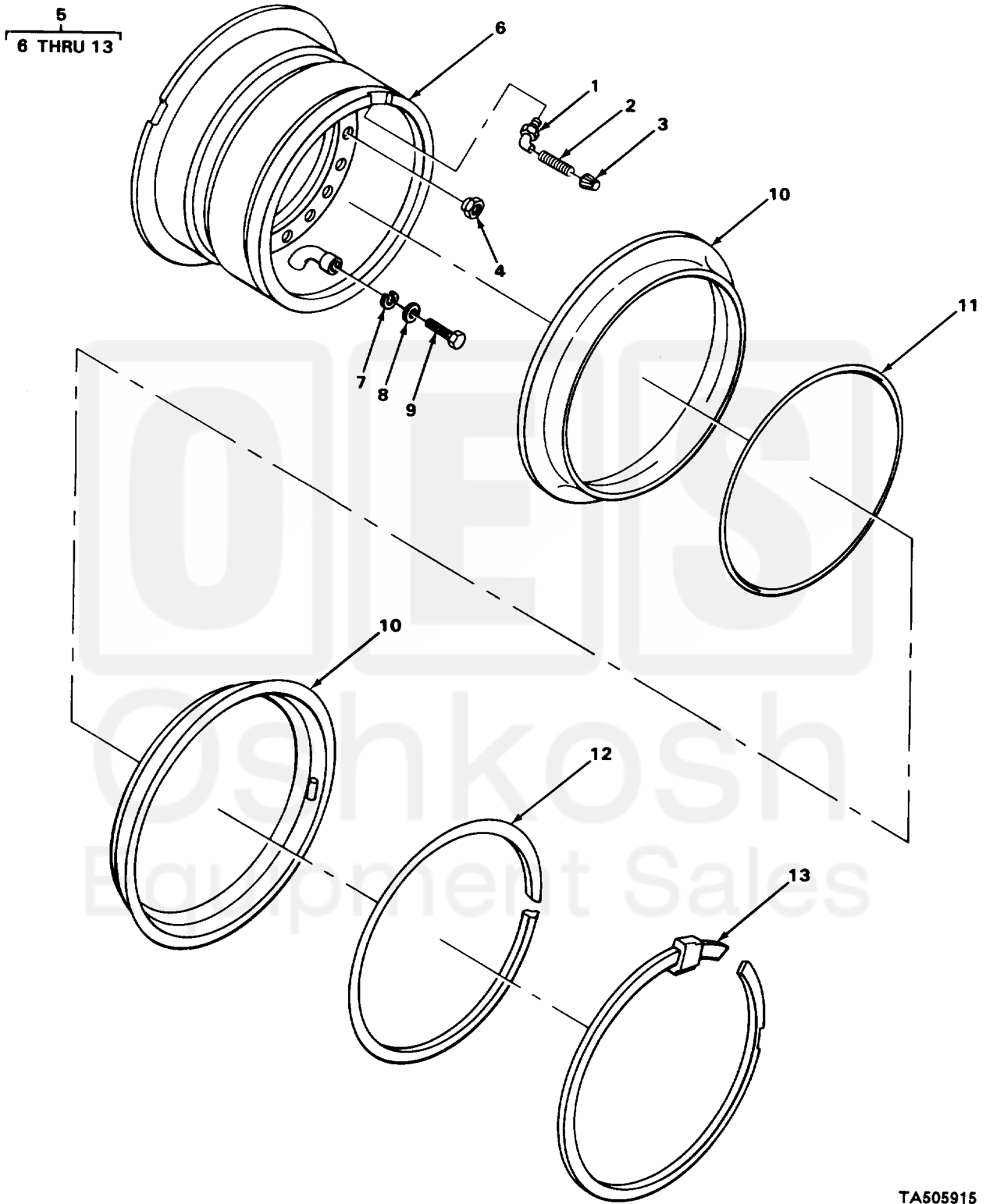
FIGURE 70. WHEEL ASSEMBLY.
