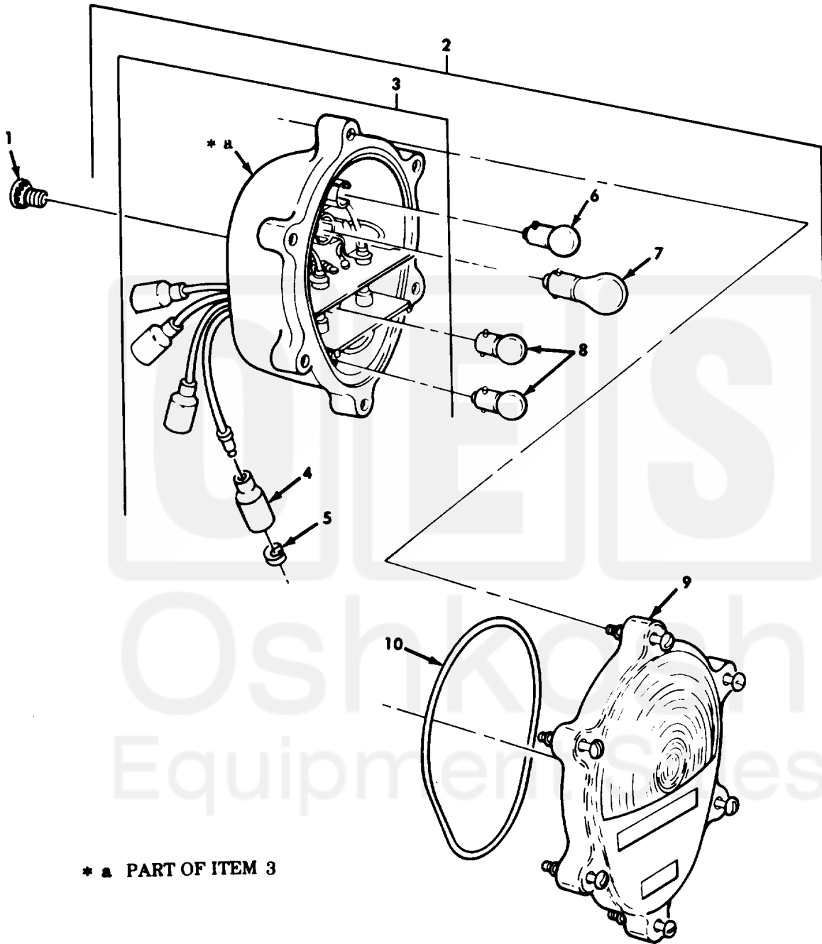
Figure 103. Taillight Assembly and Mounting Hardware.
