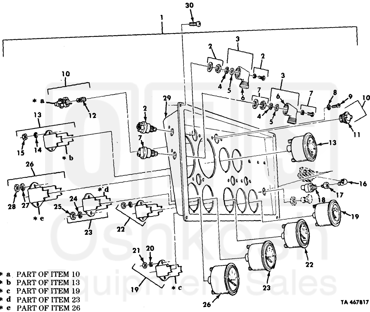
Figure 82. Instrument Cluster Assembly.
