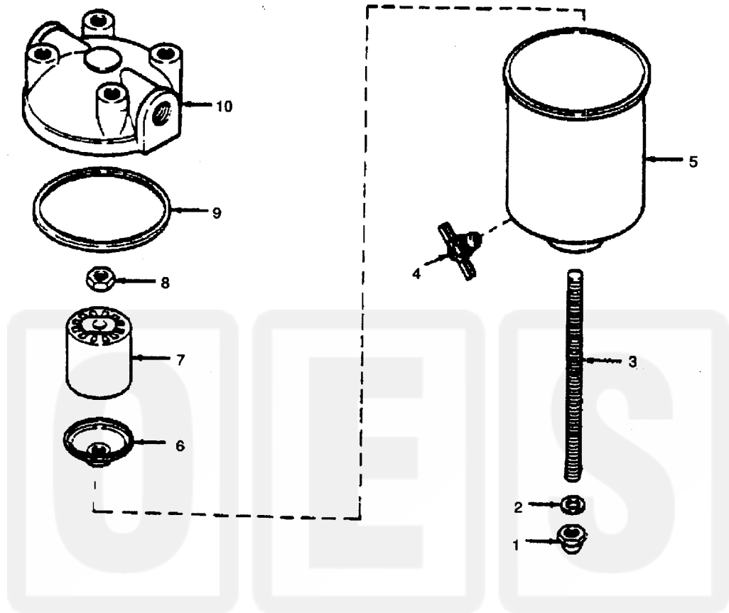
Figure 19. Fuel Strainer- Exploded View
